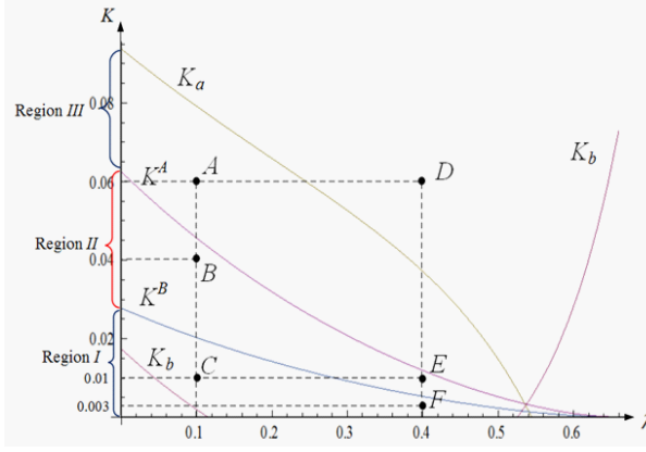
Figure A1. Low pollution intensity, \alpha = 0 .
