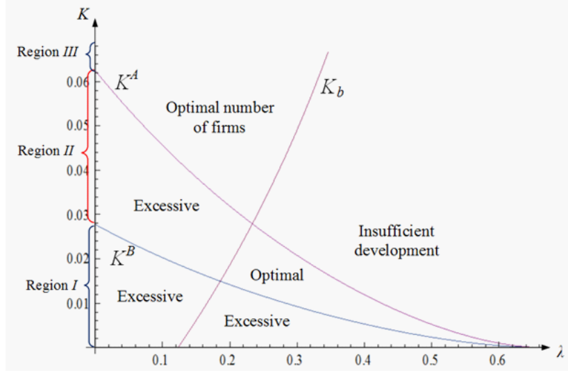
Fig 7. Insufficient and excessive development when \alpha=0.8 .
